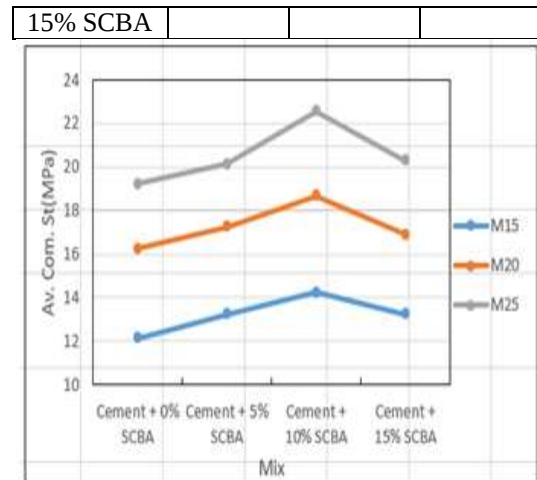
Fig 2 Av. Compressive strength (MPa) for different grade corresponding to various % of SCBA for 7 days
